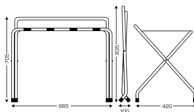
REF 8 66 506 LUGGAGE Rack S/S Chrome UPC 1
